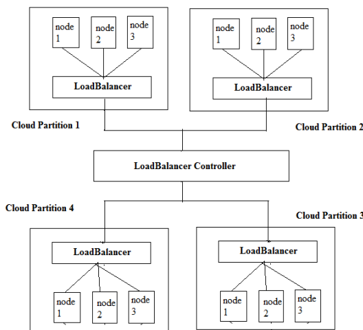
Fig. 2 Relationship between load balancer controller load balancer and nodes
